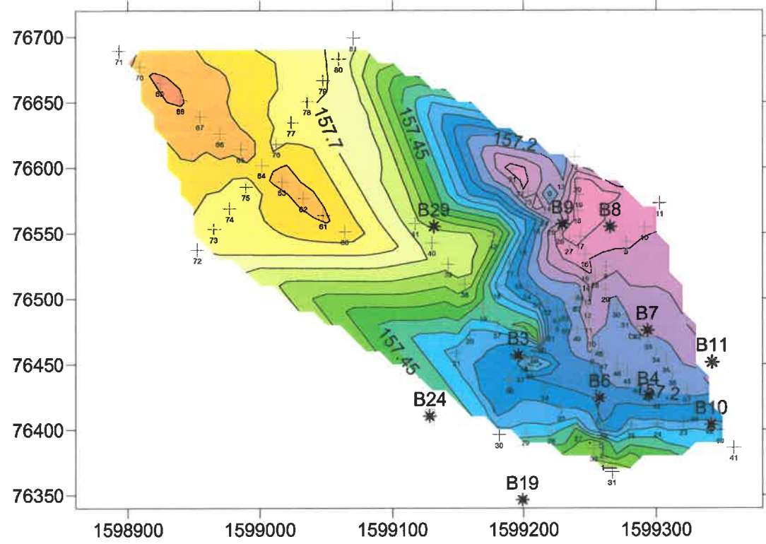
Bouguer Gravity Contour
